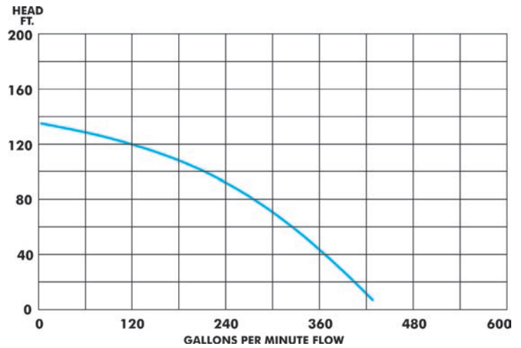
ST61460 Performance Curve 6" Discharge
