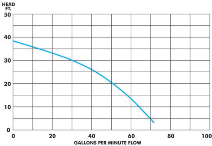
ST2037 Performance Curve 2" Discharge
