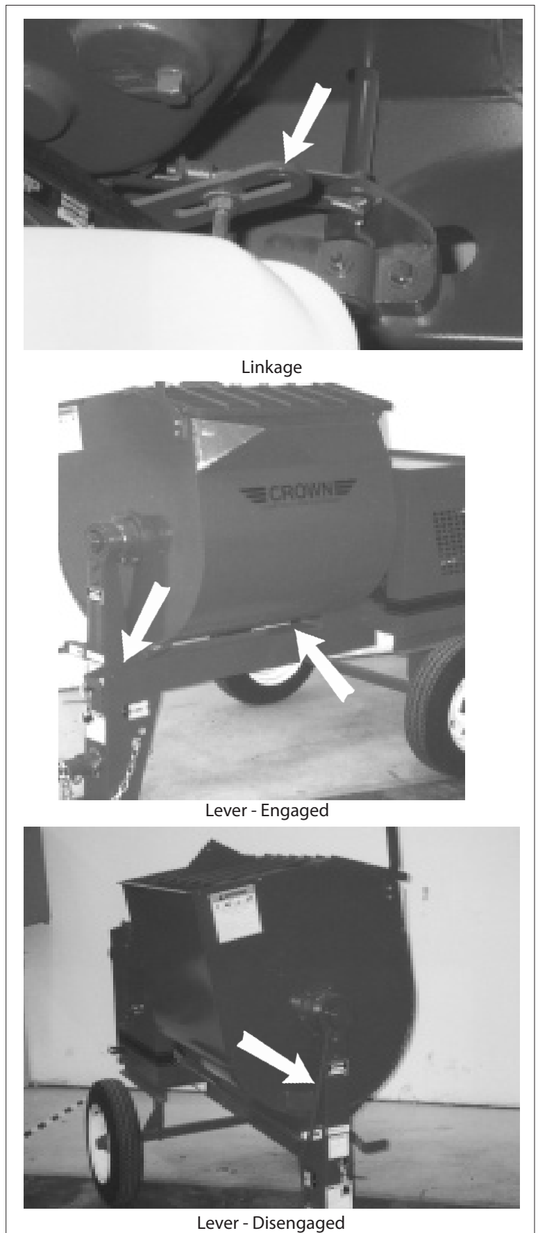
Fig. 14 POWER ENGAGING CLUTCH SYSTEM
