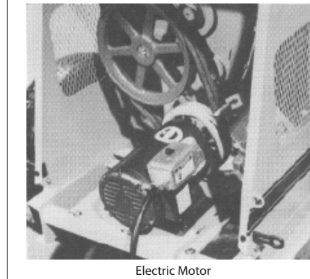
Fig. 23 DRIVE COMPARTMENT
