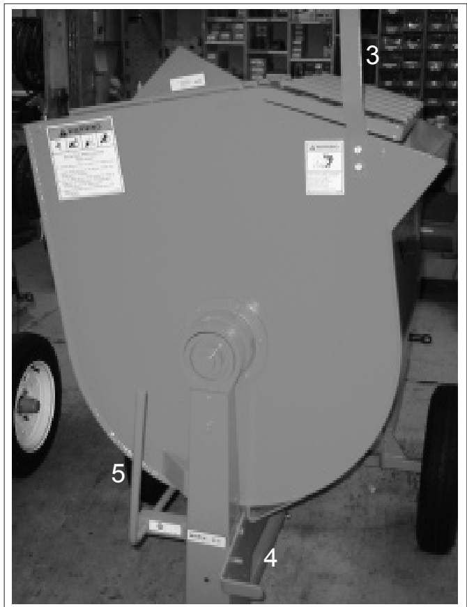
Fig. 5 DRUM EMPTYING CONTROLS
