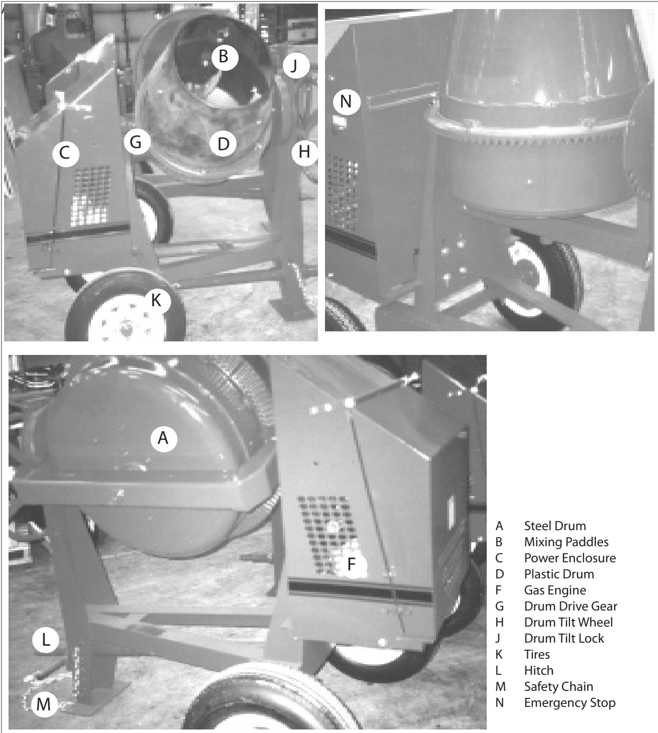
Fig. 1 MACHINE COMPONENTS
