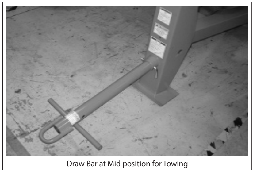
Fig. 15 ATTACHMENT
