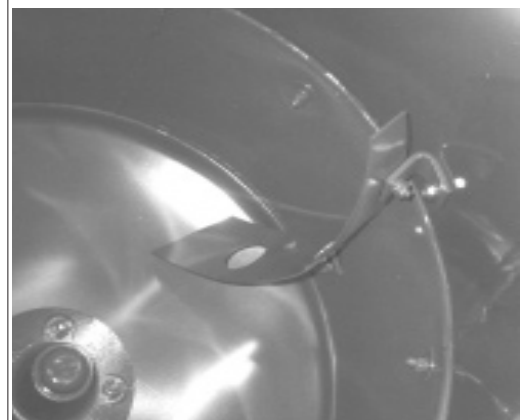
Poly Drum
