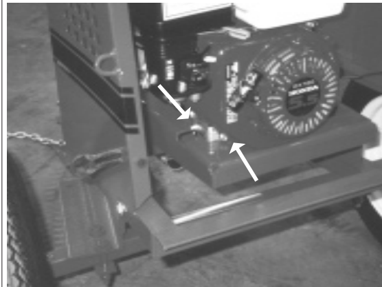
Mounting Bolts
