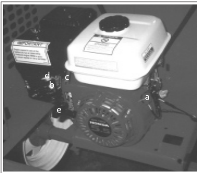
Fig. 2 GAS ENGINE CONTROLS
