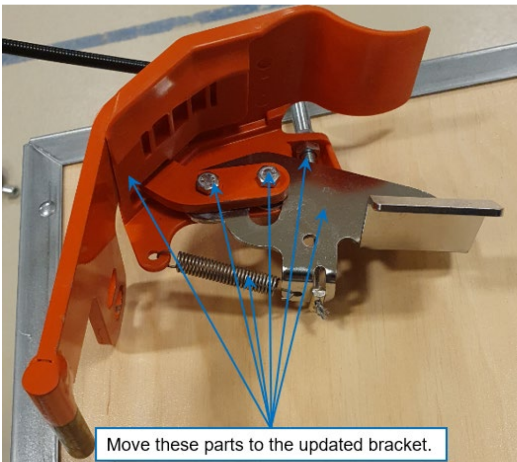
Figure 7: Parts to be moved and used with the new bracket.
