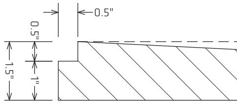
Detail Z-Z 5x
