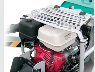
Rugged engine guard for improved protection.
