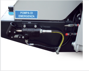
Emergency hand pump with ease of access and operation.
