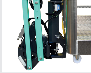
Compactness of the jib assembly hosting both the load cell and basket rotation system.
