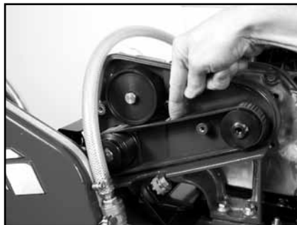
(T) Check Micro-V Belt tension (proper tension 1/8-inch).
