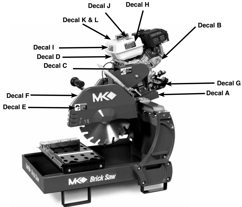
Fig. 4 MK-2000 Safety Decal Locations
