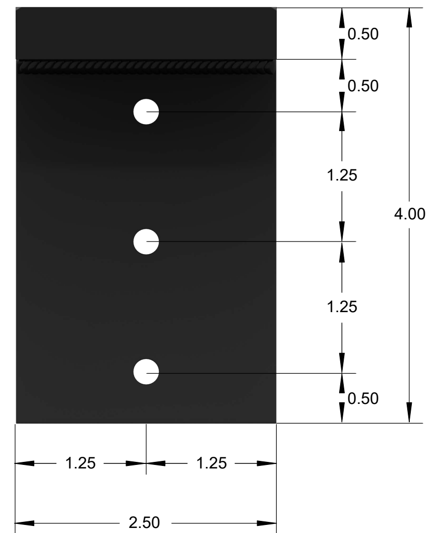
RS-W-xx-04 Front View
