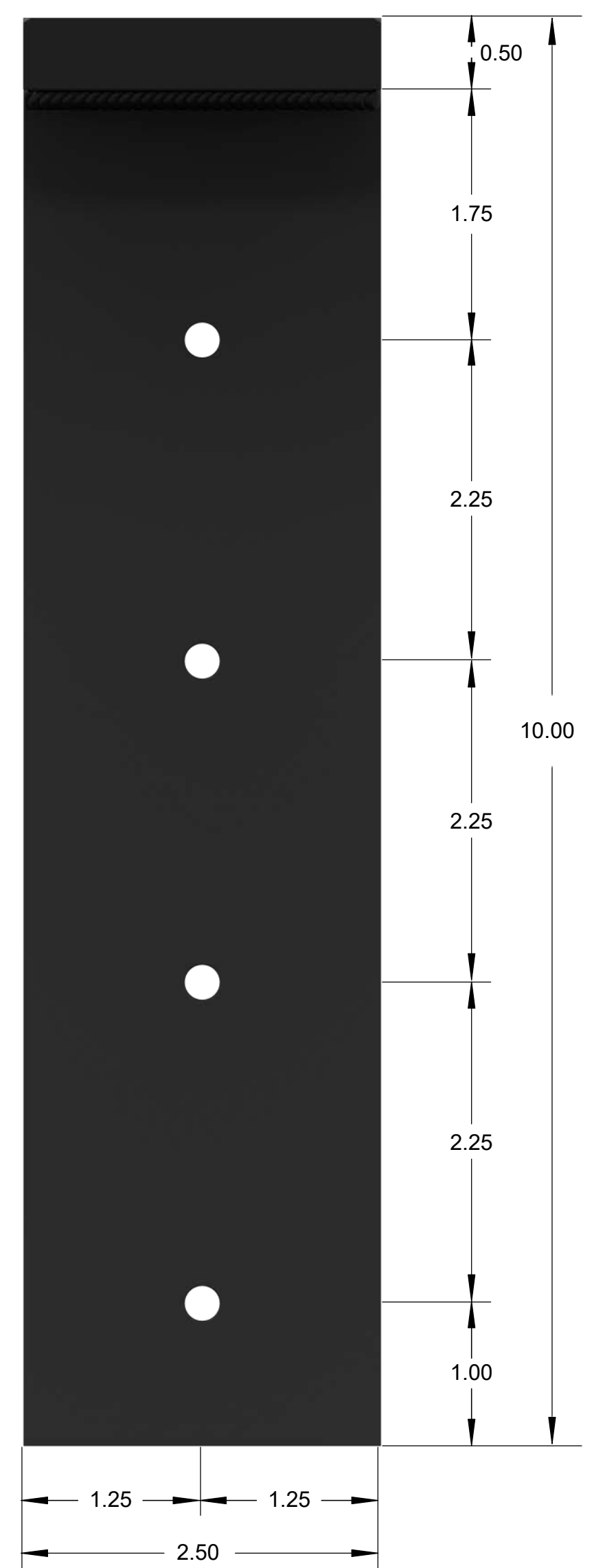
RS-W-xx-04 Front View
