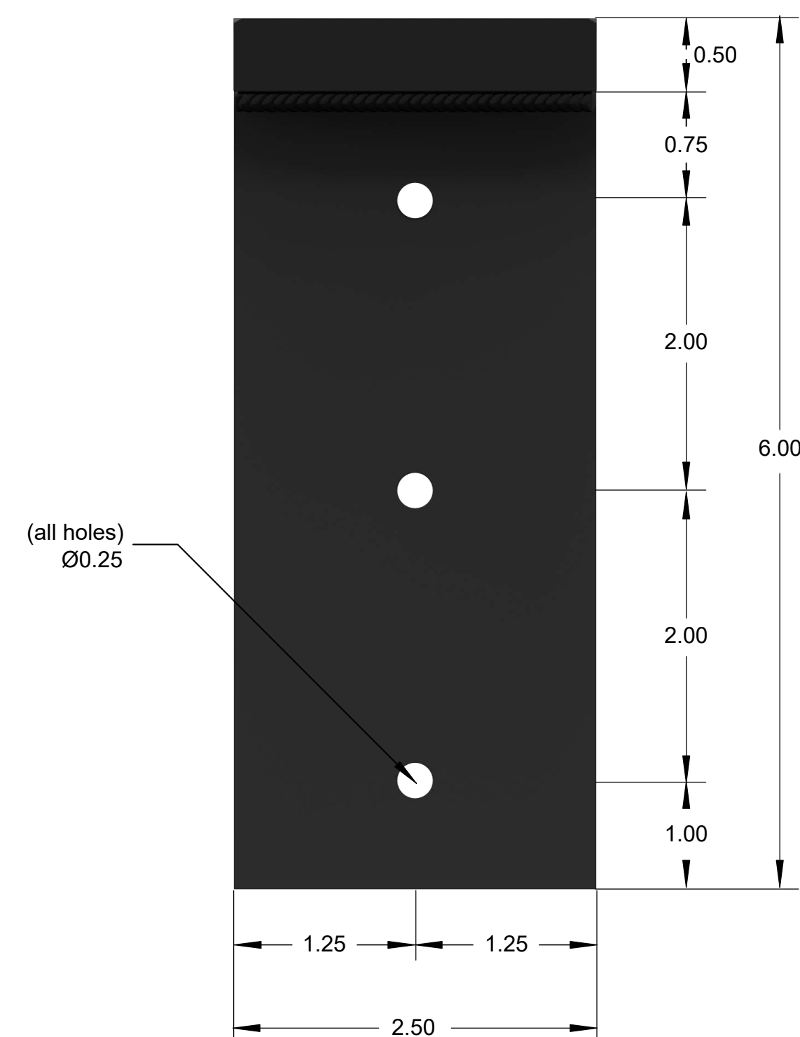
RS-W-xx-06 Front View
