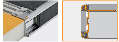
2.9 Schluter®-RONDEC-CT
