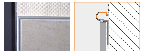
2.5 Schluter®-RONDEC-DB
