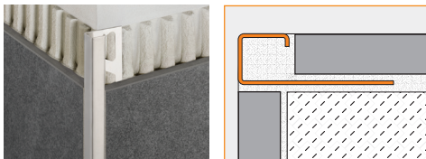
2.10 Schluter®-QUADEC
